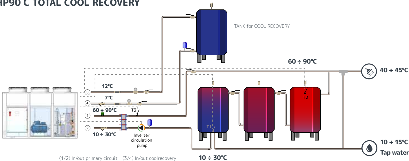
(1/2) In/out primary circuit (3/4) In/out coolrecovery
