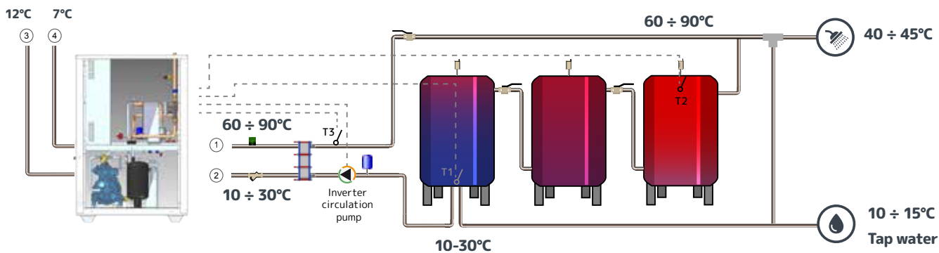
(1/2) In/out primary circuit (3/4) In/out source
