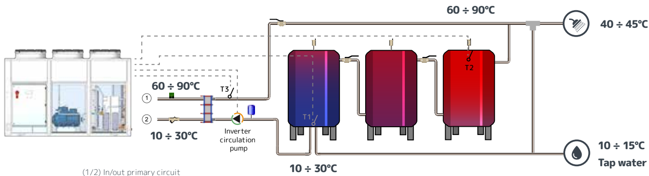
(1/2) In/out primary circuit
